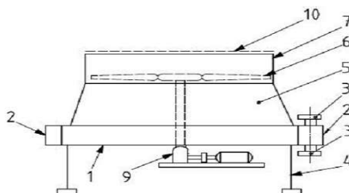
b) Induced draught
