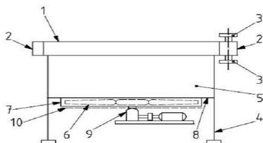
a) Forced draught
